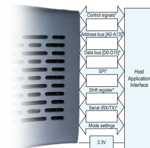
Block diagram
